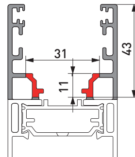
Vista Frontale Front View
