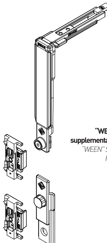
ACX.08.05 Braccio supplementare Supplementary arm
