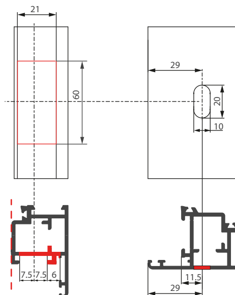
ACX.08.50 Shark - kit fissaggio art. ACX.08.52 Shark - kit for fixing ACX.08.52
